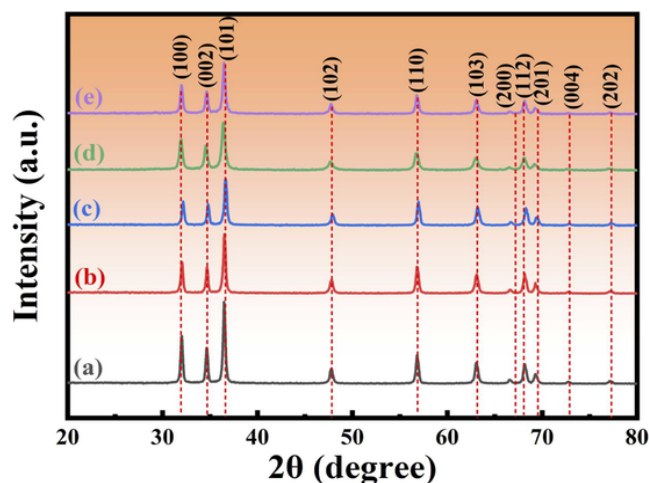
Fig. 1. X-ray diffraction (XRD) patterns of (a) pure ZnO and Sr-doped ZnO photocatalysts with varying Sr concentrations: (b) 1 wt%, (c) 2 wt%, (d) 3 wt%, and (e) 4 wt%.
