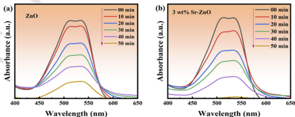
Fig. 8. UV-Vis absorption spectra of RR 120 with different irradiation time under Sunlight irradiation with (a) ZnO (b) 3 wt% photocatalysts [Catalyst dosage = 20 mg; pH = 7; Dye concentration = 50 ppm].
