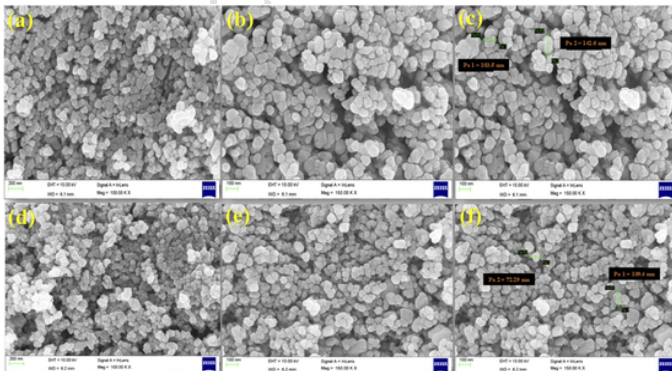
Fig. 3. FE-SEM images of (a-c) ZnO and (d-f) 3 wt% Sr-ZnO photocatalysts.
