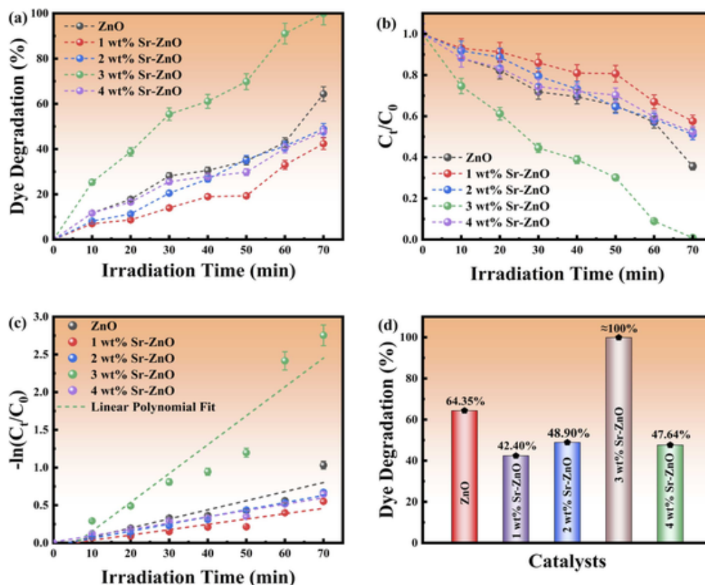
Fig. 7. (a) Photocatalytic activity results, (b) Normalized absorbance spectra ( C_t/C_0 ), (c) Kinetic linear fitting results (d) Comparison of photocatalytic activity at 70 min with, 1 wt%, 2 wt%, 3 wt% and 4 wt% Sr-ZnO photocatalysts.
