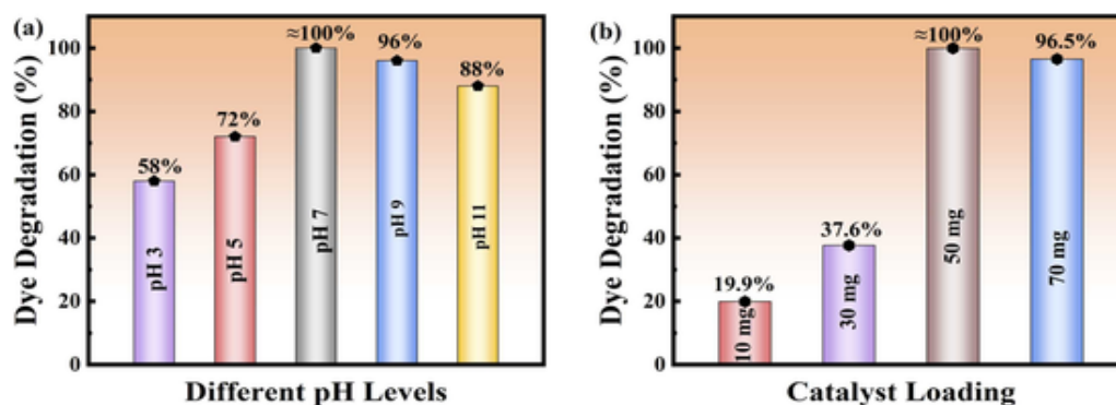
Fig. 10. (a) The effect of pH levels (using 20 mg of 3 wt% Sr-ZnO; 70-minute irradiation time). (b) Effects of catalyst dosage on photocatalytic degradation of RR 120 after 30 min of UV-A light at pH 7.
