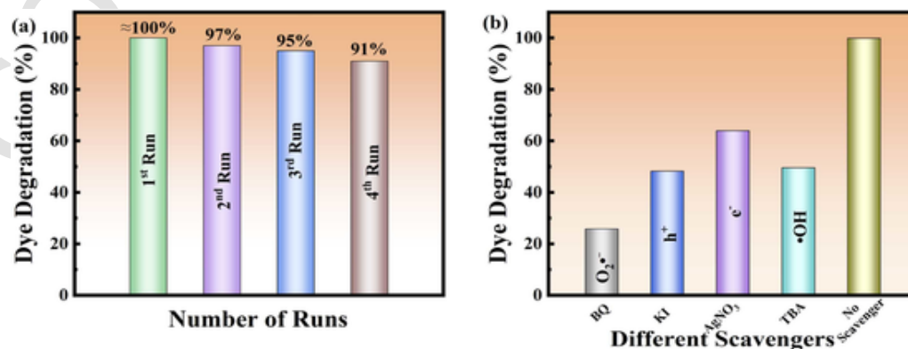
Fig. 11. (a) Reusability results (b) Effect of scavengers in pH 7 with catalyst dosage of 50 mg in RR 120 degradation under UV-A light with 30 min of irradiation.
