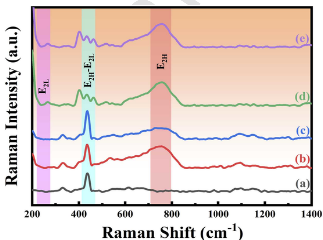
Fig. 2. FT-Raman spectra of (a) ZnO and Sr-doped ZnO photocatalysts at varying Sr concentrations: (b) 1 wt%, (c) 2 wt%, (d) 3 wt%, and (e) 4 wt%.
