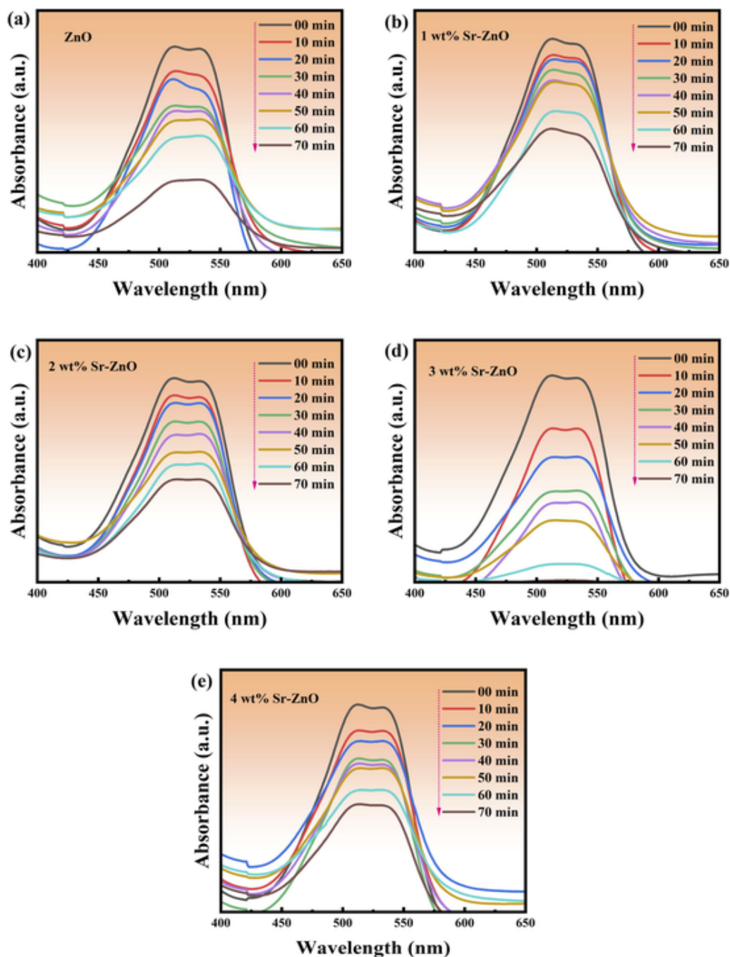
Fig. 6. UV-Vis absorption spectra of RR 120 with different irradiation time under UV-A light with (a) ZnO (b) 1 wt% (c) 2 wt% (d) 3 wt% (e) 4 wt% Sr-ZnO photocatalysts [Catalyst dosage = 20 mg; pH = 7; Dye concentration = 50 ppm].
