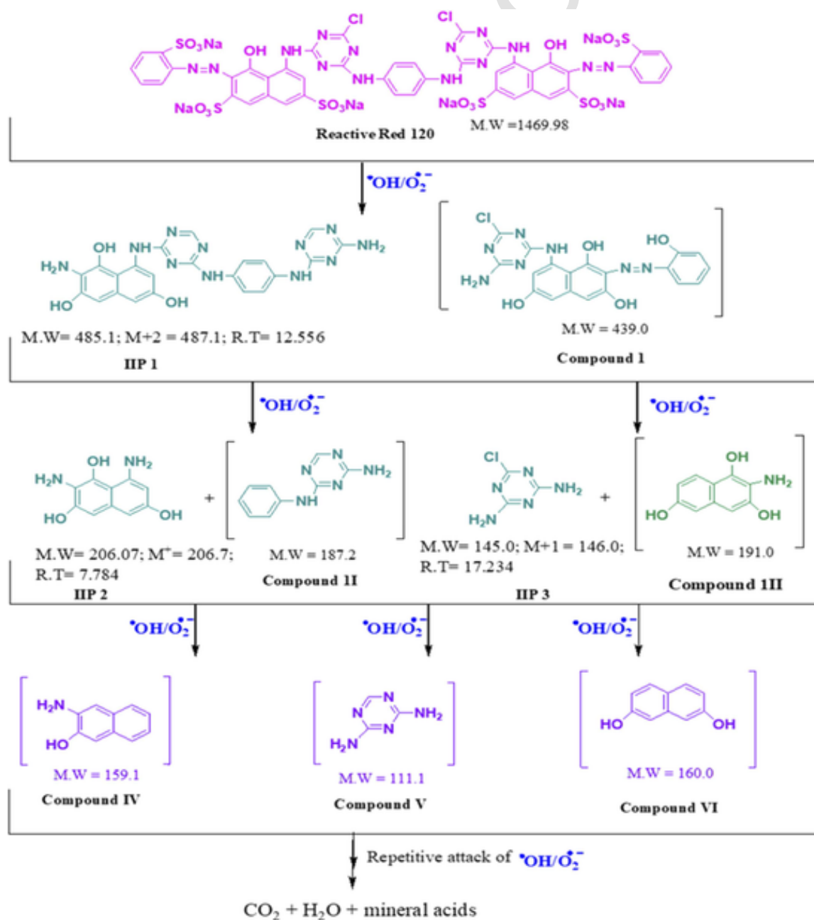
Fig. 12. Photocatalytic degradation pathway of RR 120 dye under UV-A light with Sr-ZnO.
