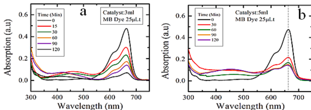
Fig. 8. Photocatalytic activity of Cu-Ag-BMNPs with Catalyst (a) 3 ml, (b) and 25 \mu Lt of MB dye (200 ml DI water).
