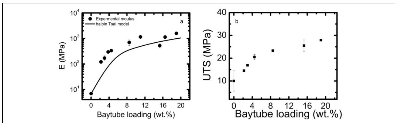
Figure 3. Mechanical characteristics of composites. (a) The values of E (black solid circles) of the composites increase by >20,000% with loading of 19 wt% of nanotubes. The enhancement in E is well-predicted by the Halpin–Tsai model (black solid line). (b) The UTS of the composites (black solid square) also increases with the loading of nanotubes. The error bars are obtained from measurements on multiple samples. E : tensile modulus; UTS: ultimate tensile strength.
