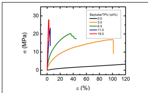
Figure 2. The tensile stress versus strain curves of TPU polymer and composites with various Baytube concentrations. TPU: thermoplastic polyurethane.
