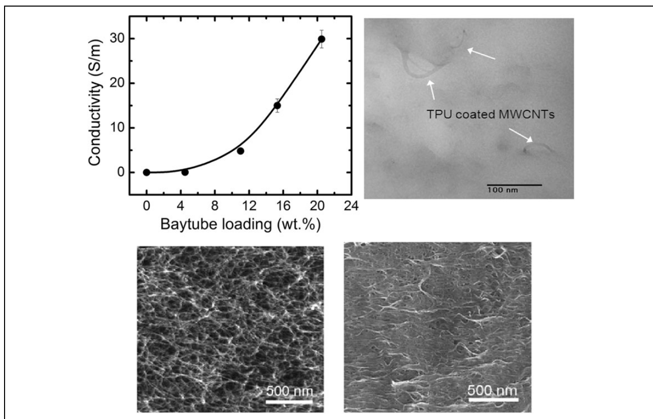
Figure 6. Electrical conductivity of aerogel-based composite scaffolds as a function of nanotubes loading (wt%) and the SEM image of CNT, TPU-coated CNTs. TPU: thermoplastic polyurethane; CNT: carbon nanotube; SEM: scanning electron microscope.
