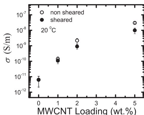
Figure 3. Electrical conductivity of neat iPP and iPP/MWCNT composites as a function of MWCNT loading (wt.%) for sheared (filled circles) and non-sheared (empty circles) composites
