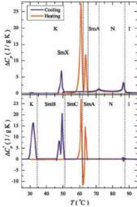
Fig. 3 — Overview of the excess reversible (top panel) and non-reversible (bottom panel) specific heat on cooling then heating between <95 and 25°C by MDSC. This excess specific heat was determined by subtracting a linear background over the entire experimental temperature range from the reversible and non-reversible specific heat. Scans were performed using parameters that most closely approximated static heat capacity results; a base scan rate of \pm 0.3 K/min and an induced temperature amplitude of 0.5 K at 120 s heating period. Note that the cooling scan was paused at 47°C (320.2 K) for <2 h before continuing.
