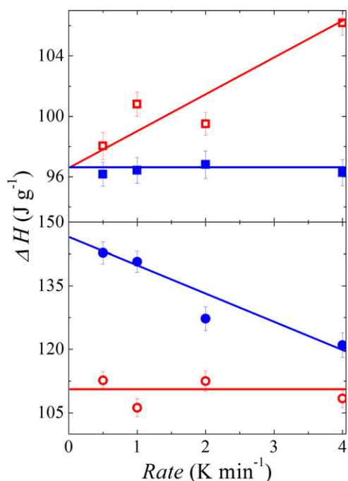
Figure 9. The total effective transition enthalpy as function of scan rate for neat iPP [top panel: cooling (■) and heating (□)] and for the 2 wt % iPP/CNT sample [bottom panel: cooling (●) and heating (○)]. Lines are guides to the eye. [Color figure can be viewed in the online issue, which is available at wileyonlinelibrary.com .]
